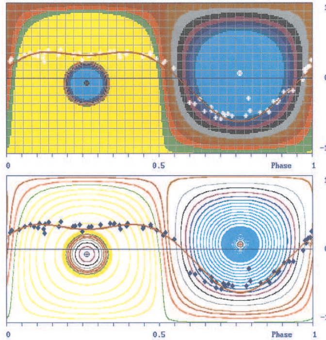
Fig. 6. Magnetic map with phase curve of the observations. Top: Map-phase-diagram with colored magnetic isolines differently arranged to Fig. 5 because of the ring-like covering. Bottom: Representation of the map in form of isolines, which gives an impression on field structure and polarity related to the phase curve with the dots of the observations.
