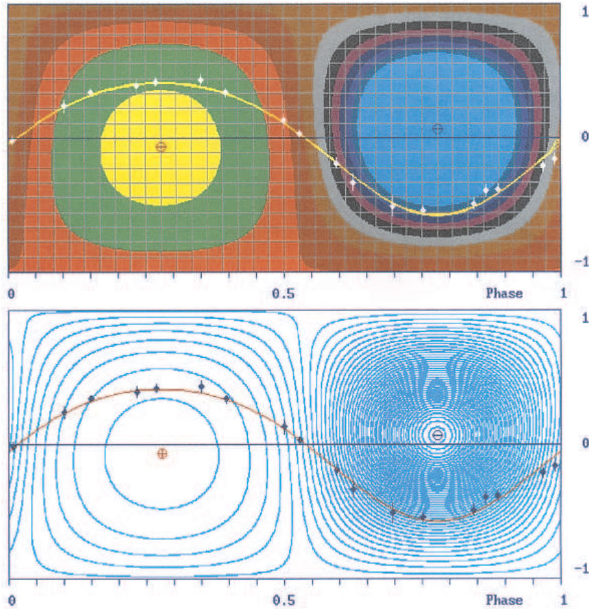
Fig. 4. Fitting of the photoelectrical observations of Borra and Landstreet.
