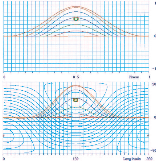
Fig. 1. Series of phase curves produced by a spot-like radiating point on the surface. Parameter of the series is the inclination angle i . From below to above: i = 135^\circ, 105^\circ, 90^\circ, 75^\circ, 60^\circ, 45^\circ, 30^\circ . Top: Brightness phase curves of a single bright spot (emission). Bottom: Magnetic phase curves of a spot on the pole. The total field is indicated by magnetic iso-lines.
