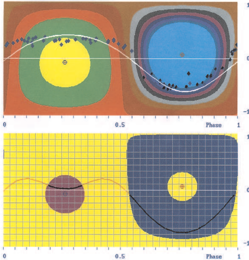
Fig. 5 Insertion of Babcock's observational data in the map/phase diagram obtained by means of Borra's and Landstreet's photometric data.
