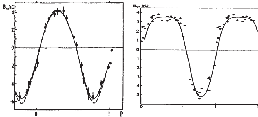
Fig. 3 Observed effective magnetic field strength B_{\text{eff}} of 53 Cam
