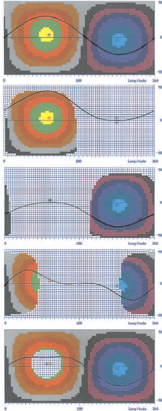
Fig. 2. Demonstration of the effect of covering parts of the surface of a magnetic star onto the phase curve.
