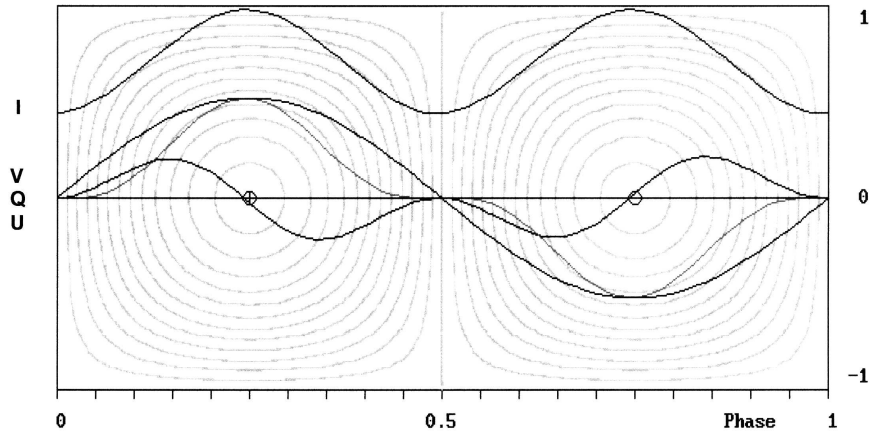
Fig. 4. Phase curves of STOKES I, Q, U, V for a magnetic dipole.
